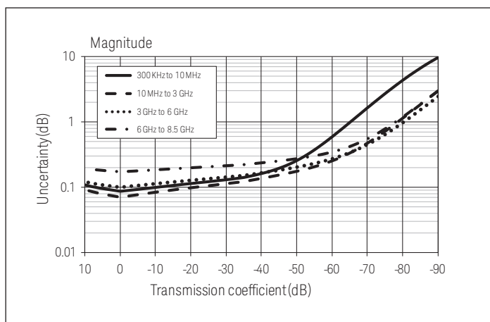
Figure 4. Transmission uncertainty (Specification)
